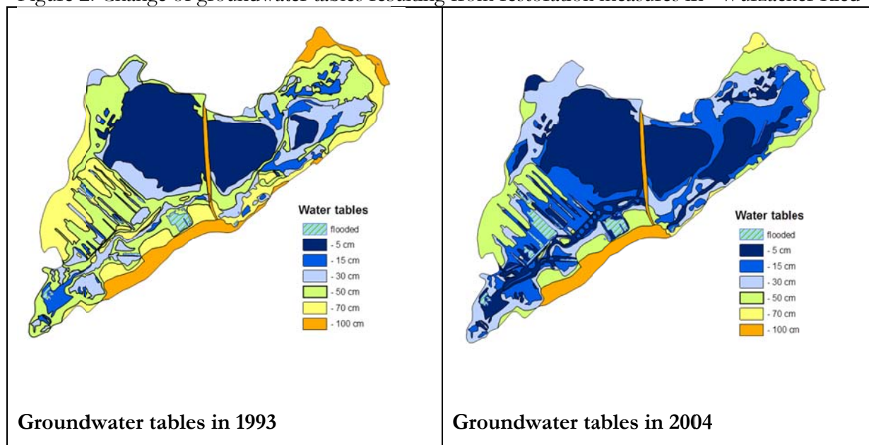
Figure 2: Change of groundwater tables resulting from restoration measures in “Wurzacher Ried”
