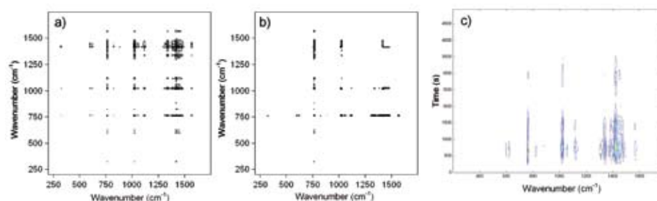
Figure 3: The synchronous plot (a), the asynchronous plot (b) and the moving window plot (c) for the low wavenumber region of the bmimBF 4 Raman spectra
