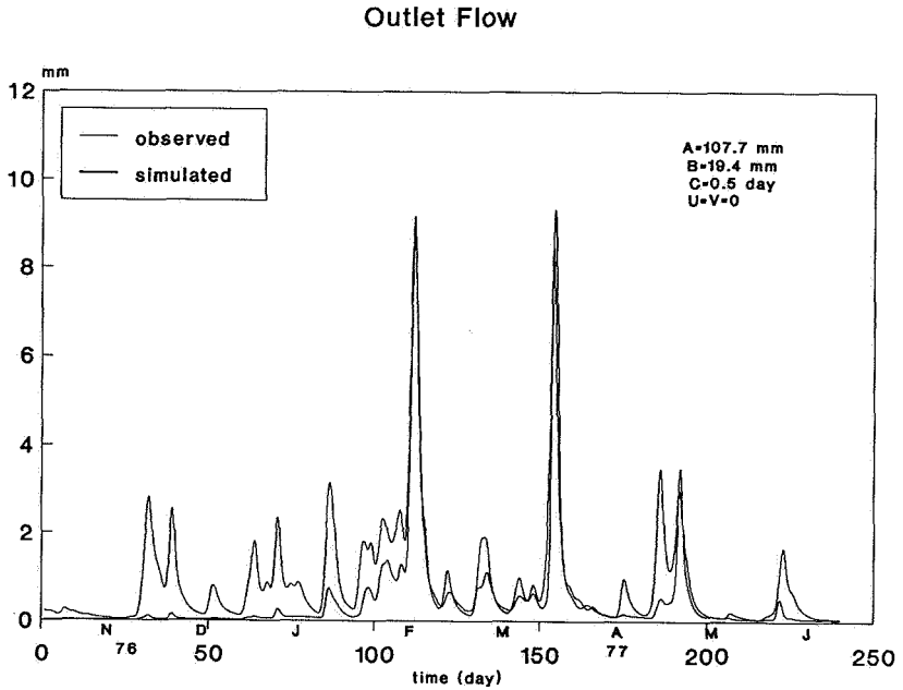
Figure 3. Outlet Flow
