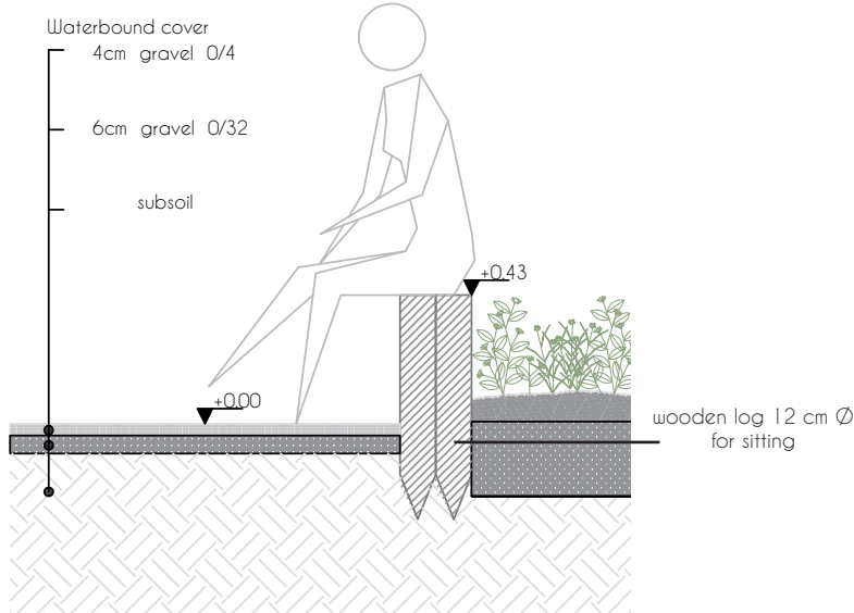
Standard details S1 M 1:25
