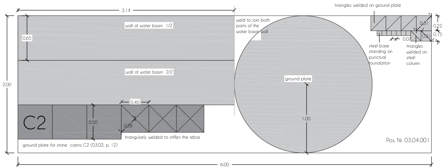
Steel panel cutting thickness 4mm M 1:25
