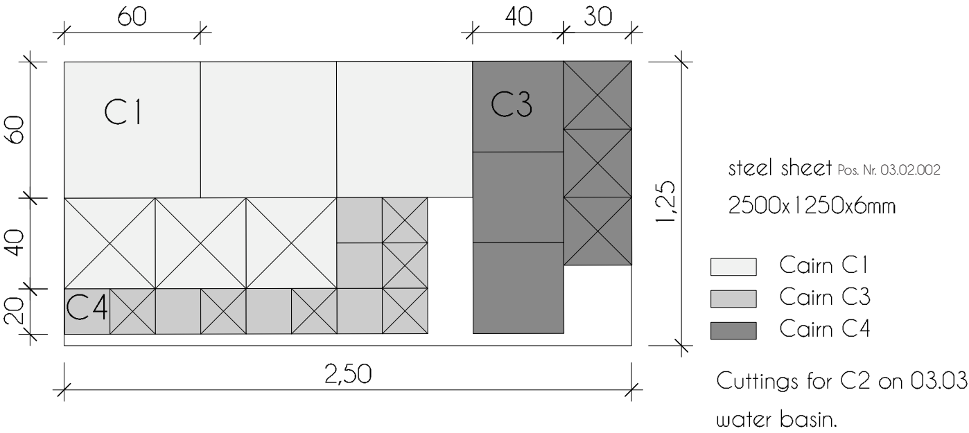
Steel panel cutting thickness 6mm M 1:25
