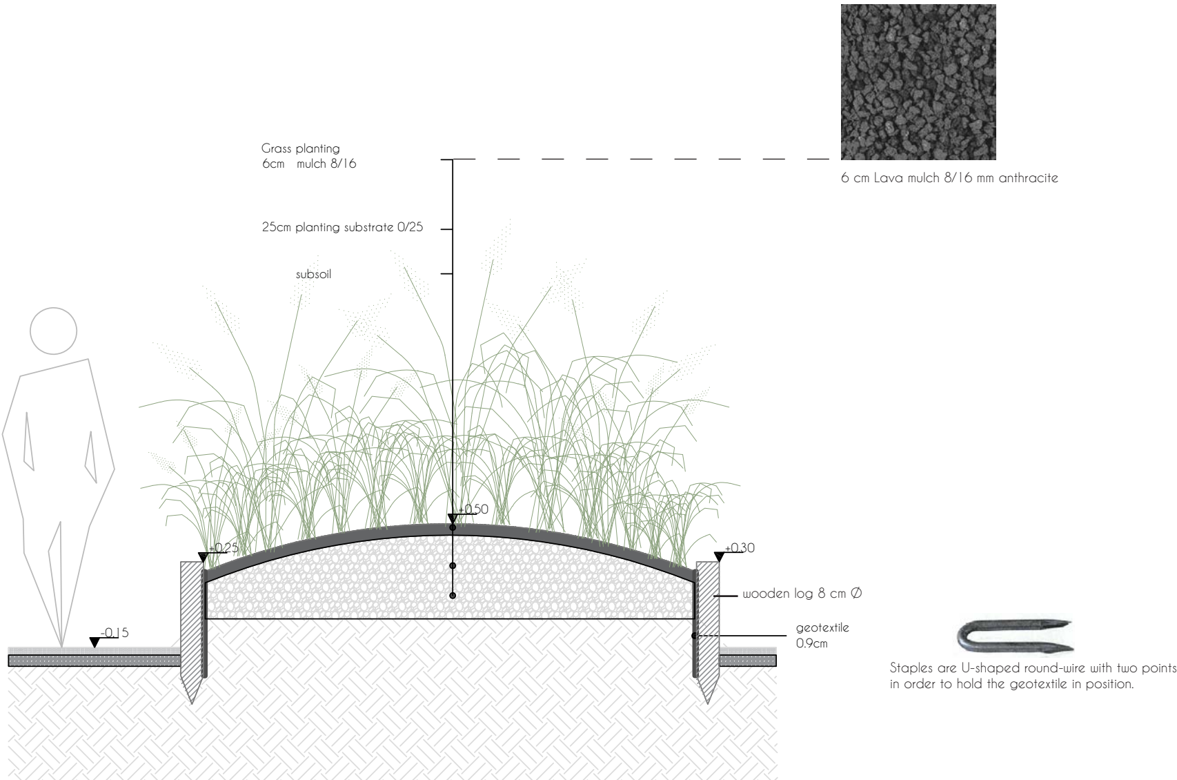
Wooden fences S2 M 1:25
