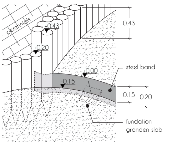
Steel transition black circle waterbound cover wood fence M 1:25
