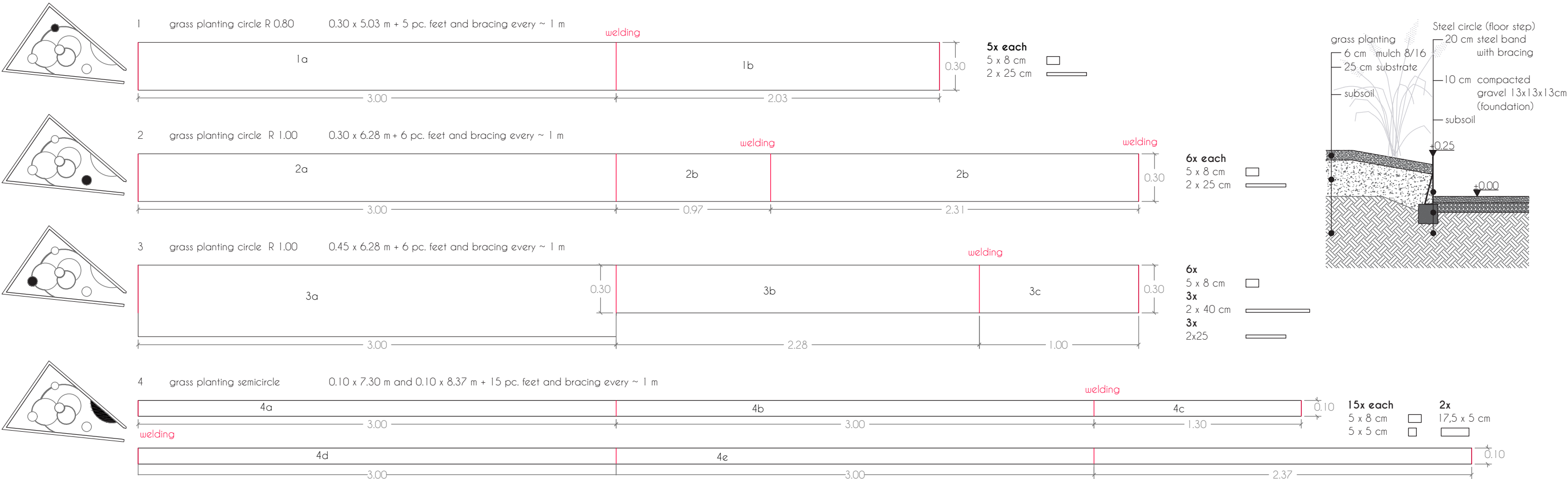
Steel circles M 1:25
